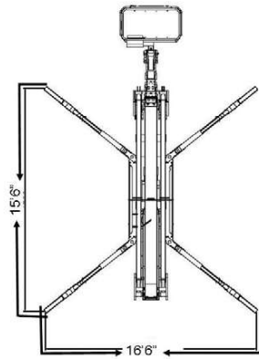
(Standard Outrigger Layout)
