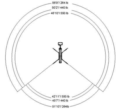
(Standard Outrigger Layout)
